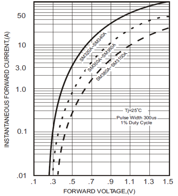
FIG.2-TYPICAL FORWARD CHARACTERISTICS
