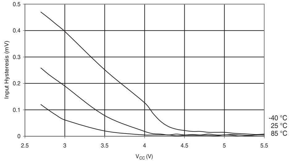
Figure 28-56. Reset Input Pin Hysteresis vs. V_{CC}
