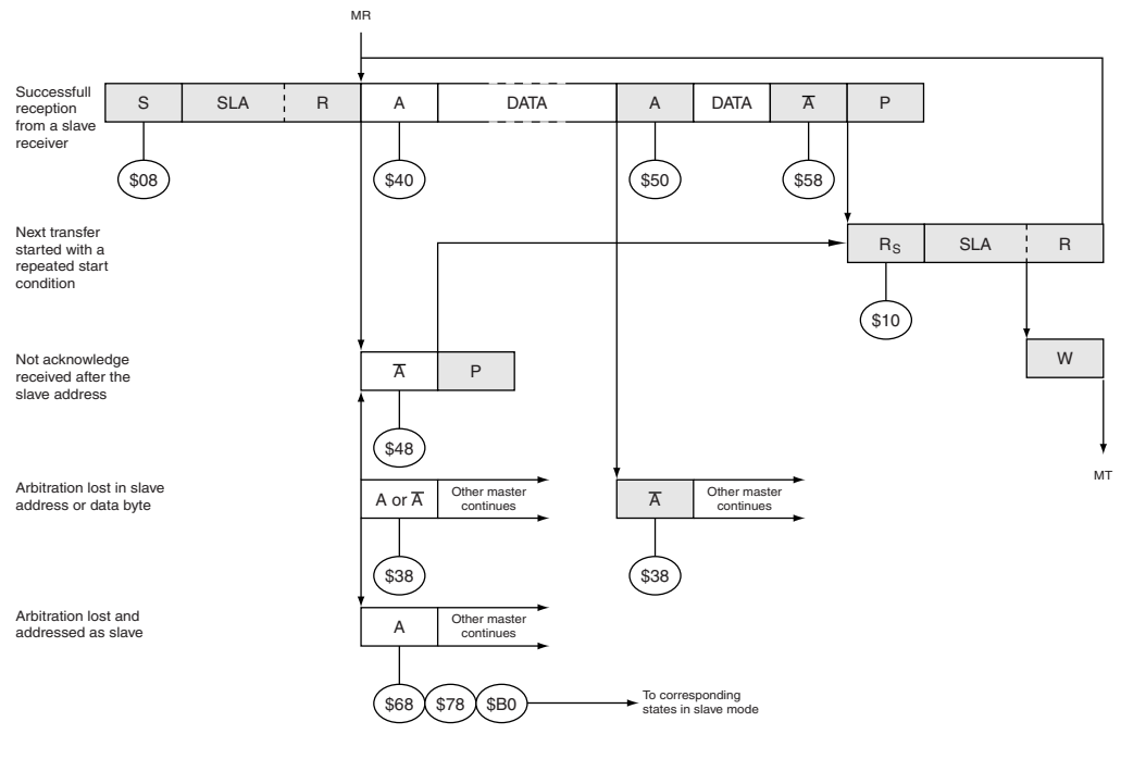
Figure 21-14. Formats and States in the Master Receiver Mode
