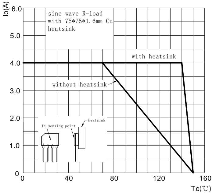
FIG1:Io-Tc Curve
