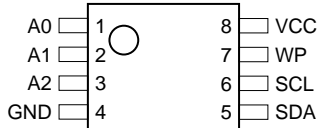
8-Pin TSSOP
