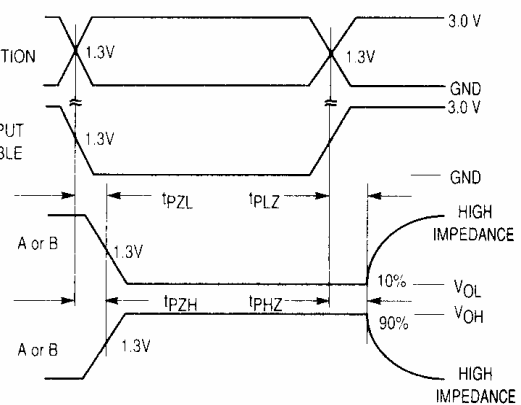
Figure 2. Switching Waveforms
