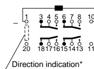
Schematic (Bottom view)
