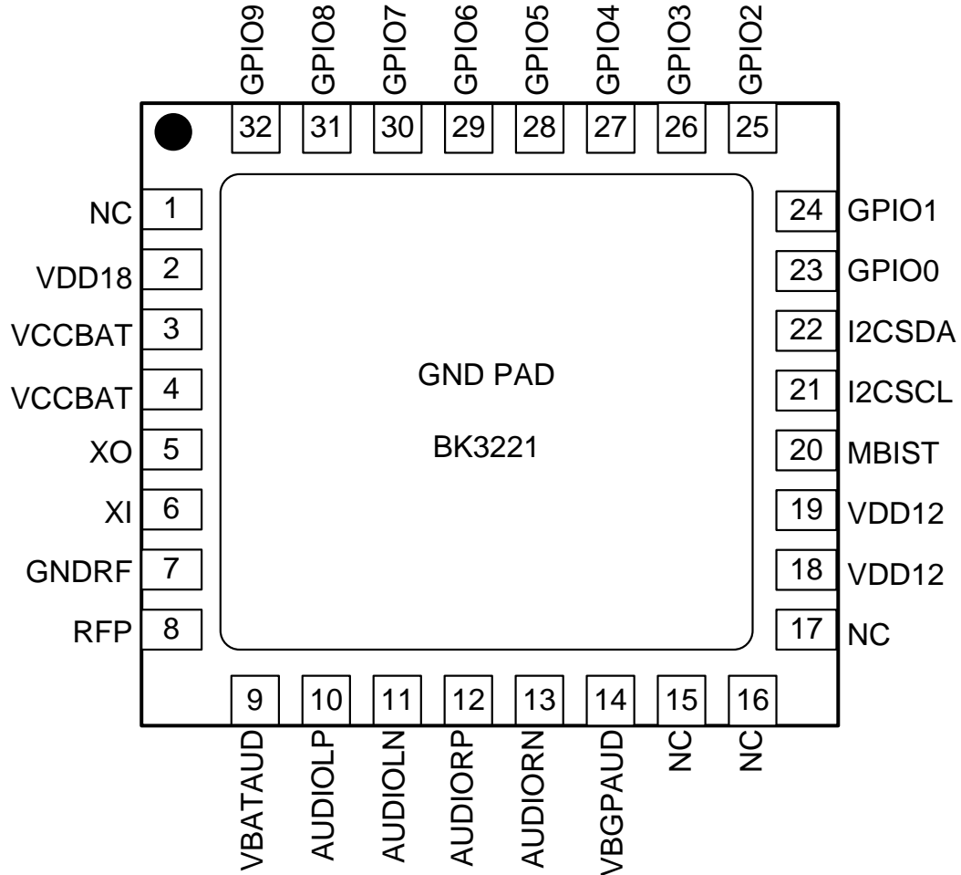
Figure 1 BK3221 PIN Definition Diagram
