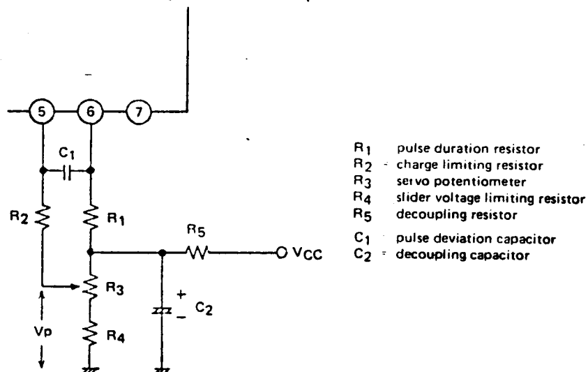
Fig. 3 Monostable set up
