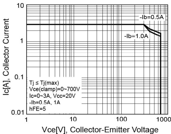
Figure 5. Reverse Bias SOA
