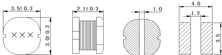
Land Pattern
