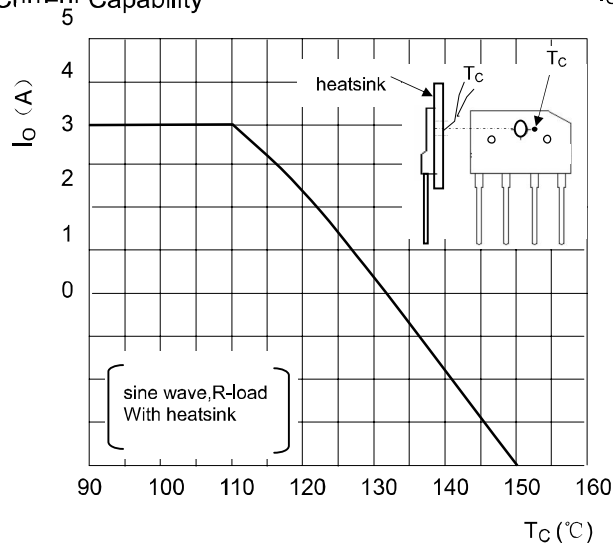
I_o - T_c Curve
