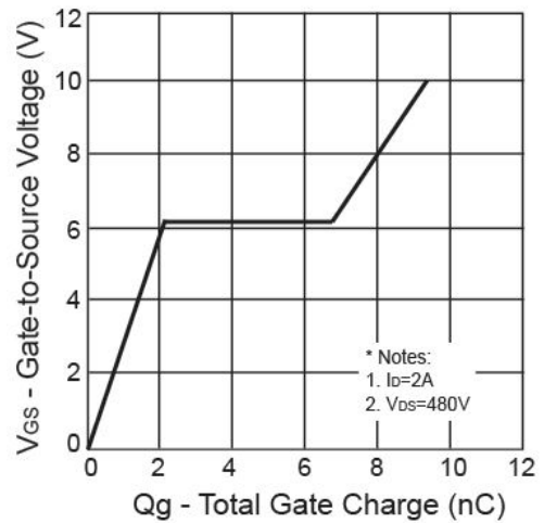
Gate Charge
