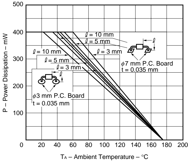
Fig. 6 POWER DISSIPATION vs. AMBIENT TEMPERATURE
