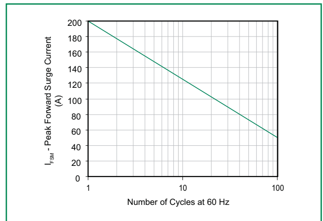
Figure 6 - Maximum Non-Repetitive Peak Forward Surge Current for Uni-Directional Only
