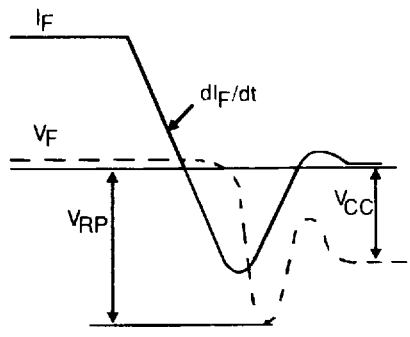
Figure 2 : Turn-off switching characteristics (with series inductance).
