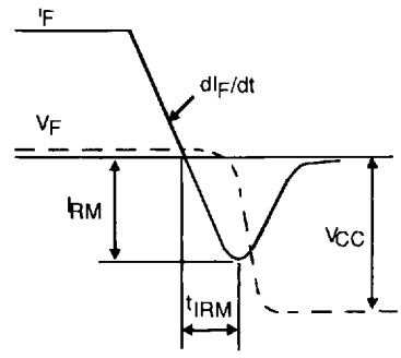
Figure 1 : Turn-off switching characteristics (without series inductance).
