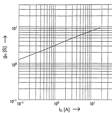
Typical Forward Transconductance vs. I_D g_{fs}=f(I_D); 80\mu s pulse test; V_{DS}=25V; T_C=25^\circ C
