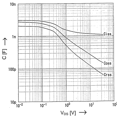
Typical Capacitances vs. V_{DS} C=f(V_{DS}); V_{GS}=0V; f=1MHz
