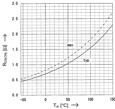
Drain-Source On-State Resistance vs. T_{ch} R_{DS(on)}=f(T_{ch}); I_D=4.5A; V_{GS}=10V
