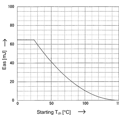
Avalanche Energy Derating E_{as}=f(\text{starting } T_{ch}); V_{CC}=60V; I_{AV}=10A
