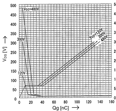
Typical Gate Charge Characteristic V_{GS}=f(Q_g); I_D=10A; T_C=25^\circ C
