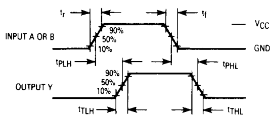
Figure 1. Switching Waveforms
