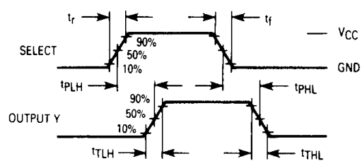
Figure 2. Switching Waveforms
