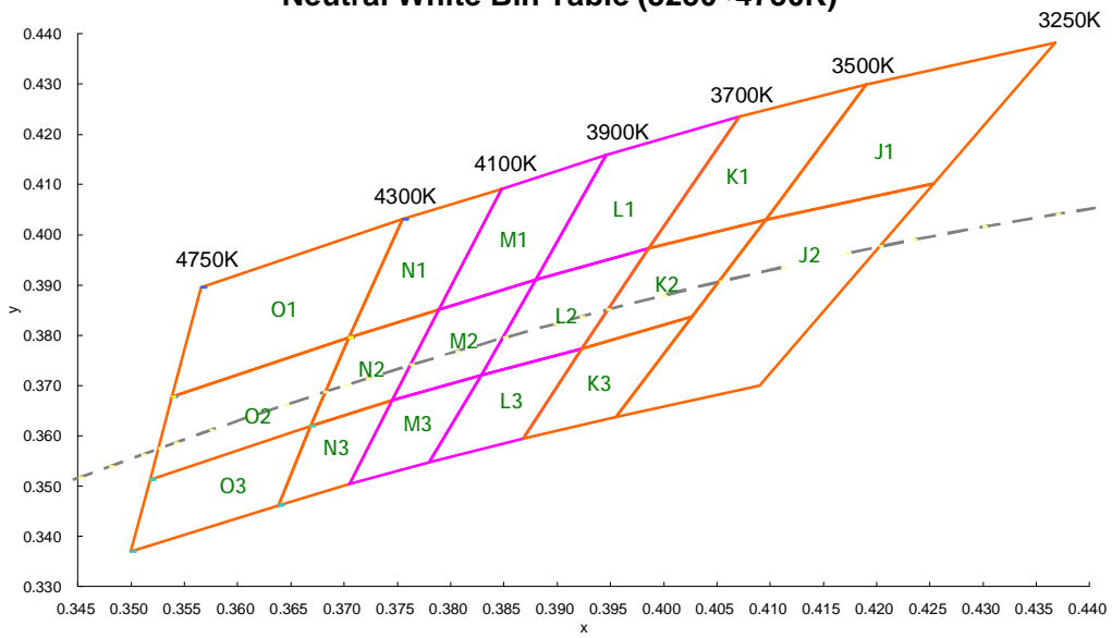
Neutral White Bin Table (3250~4750K)
