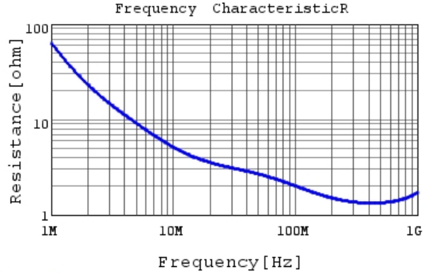
DE1B3KX101KB4BN01F R DC0V, 20degC
