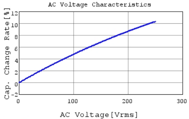
DE1B3KX101KB4BN01F C-AC Voltage capchange, I
