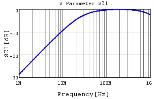
DE1B3KX101KB4BN01F S21 DCOV, 20degC
