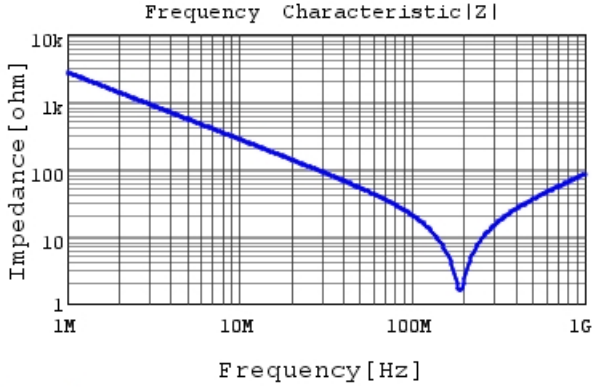
DE1B3KX101KB4BN01F |Z| DC0V, 20degC
