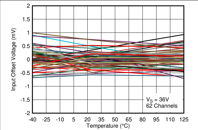
Figure 7-10. Input Offset Voltage vs. Temperature at 36V
