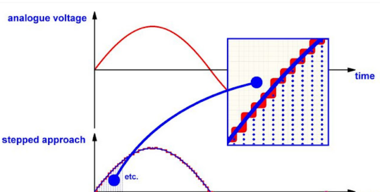
The principle of the stepped approach of the output voltage. (© 2018 Jos Verstraten)
