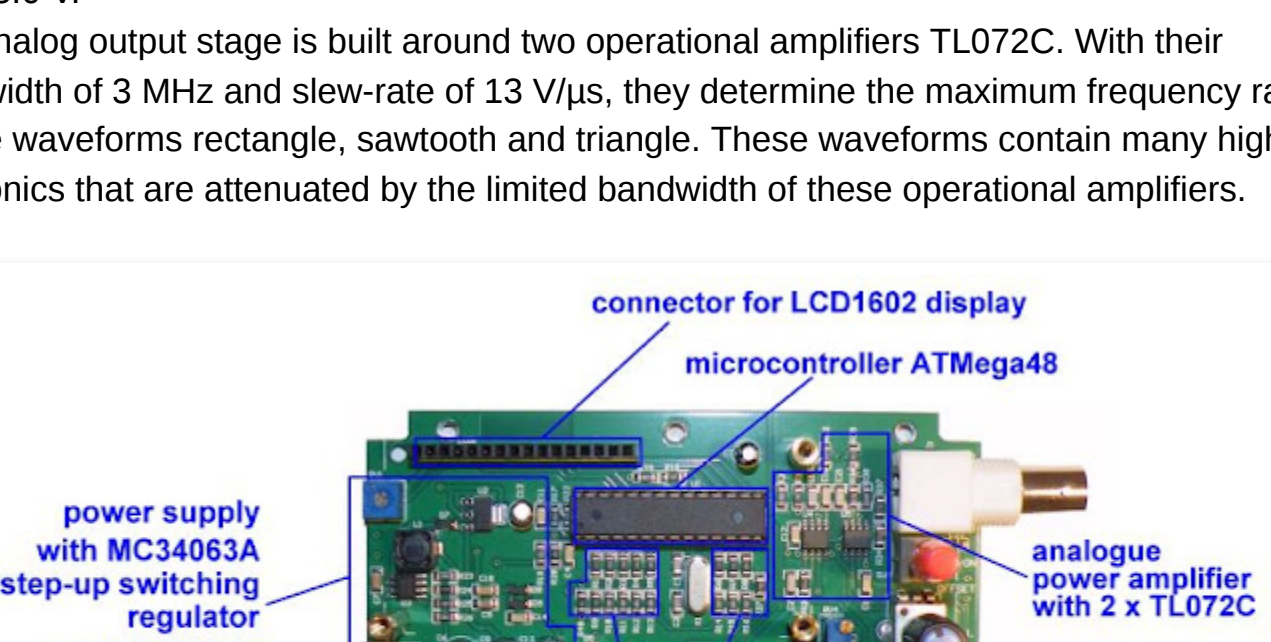
The PCB of the FG-100 contains three clearly distinguishable functional parts. (© 2018 Jos Verstraten)
