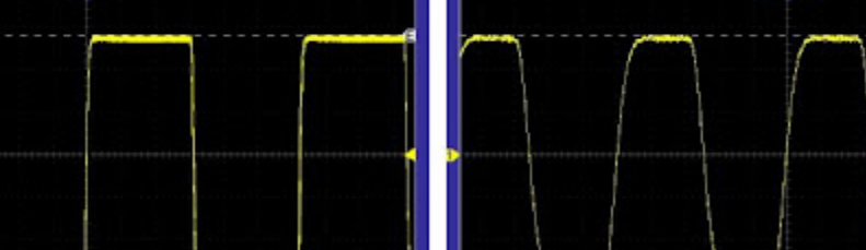
Measurement of the rise time of the leading edge of the rectangular output voltage. (© 2018 Jos Verstraten)
