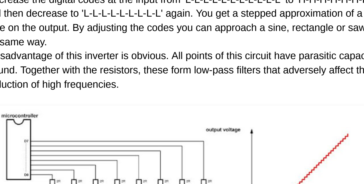
The basic circuitry of an R-2R digital to analog inverter. (© 2018 Jos Verstraten)
