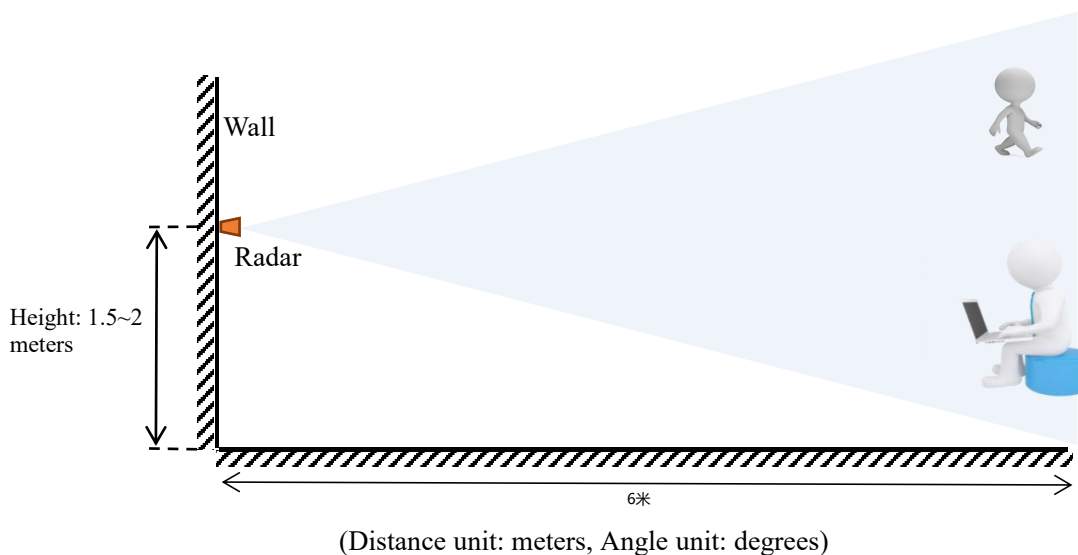
Figure 9 Schematic Diagram of Wall-mounted Installation
