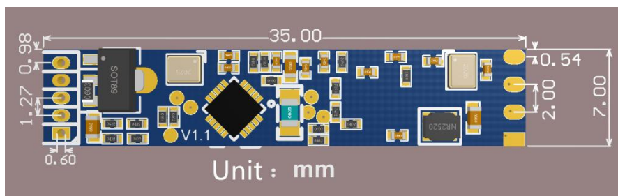
Figure 5 Module Dimensions
