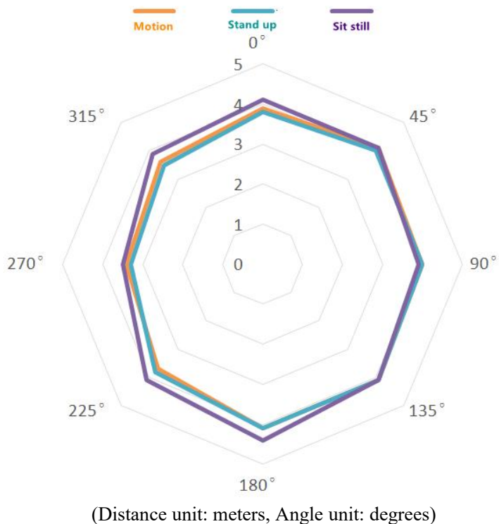
Figure 8 Schematic Diagram of the Detection Range (the ceiling height is 3 meters)
