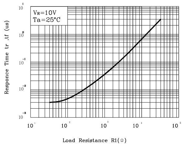
Fig. 6 Responce Time vs Load Resistance
