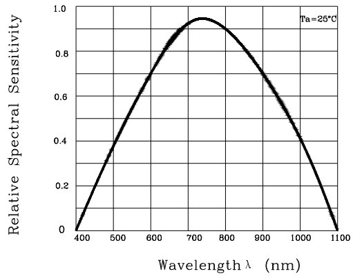
Fig. 2 Spectral Sensitivity
