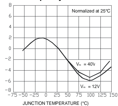
Oscillator Frequency
