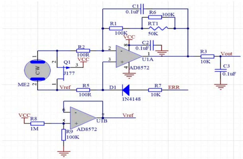
Fig2. Test circuit
